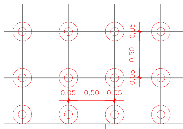
Detall A e:1/25
